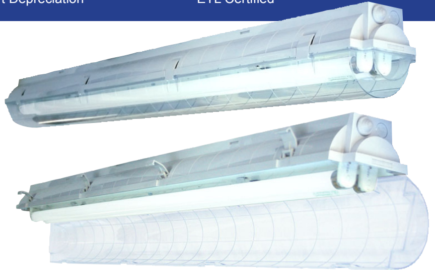
Pictured: VCO 2-Lamp T8 Fixture Optically Clear Lens 5.37" x 9.00" x 51.75"
